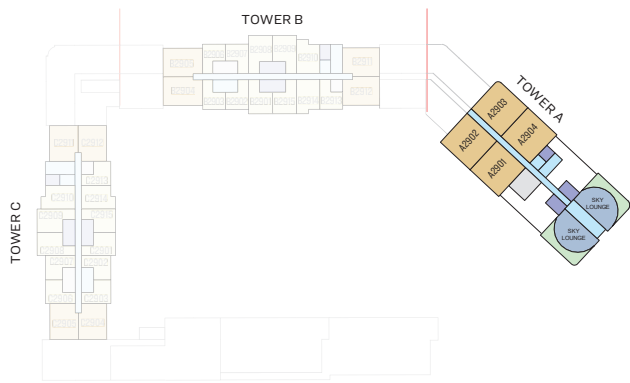
LEVEL 29
